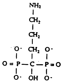
Alendronate
